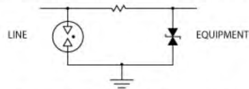
HYBRID MODELS (Standard and Heavy Duty Protection schematic per wire)
