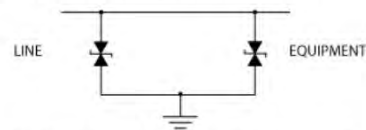
Silicon Avalanche Diode only models (Standard and Heavy Duty Protection schematic per wire)
