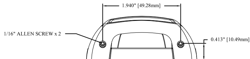
End View:
