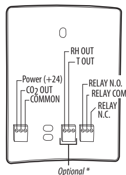
CWL: CO 2 , RH, Temperature Transmitter Options
