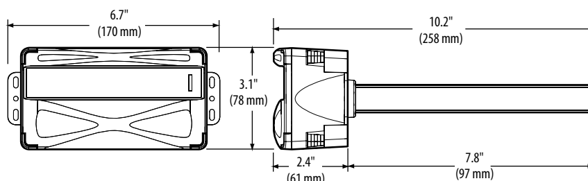
CDL Duct Mount
