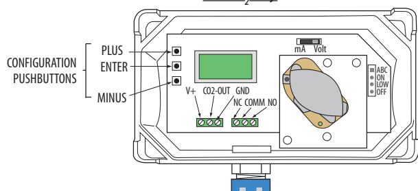
CWL: CO 2 , RH, Thermistor, Pushbutton Override, and Relay Options
